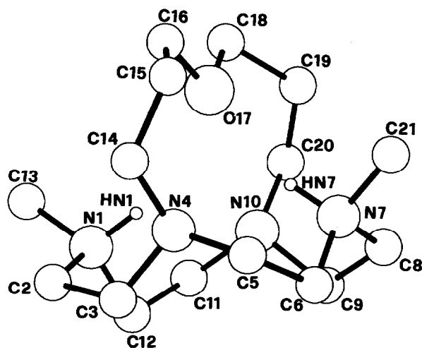
Fig. 5. Drawing of the [\text{H}_2\text{C}_3]^{2+} cation. Atomic coordinates taken from ref. 36.
