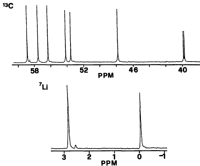
Fig. 8. ^{13}\text{C} (top) and ^7\text{Li} (bottom) NMR spectra of [\text{LiC6}]^+ complex in aqueous solution.
